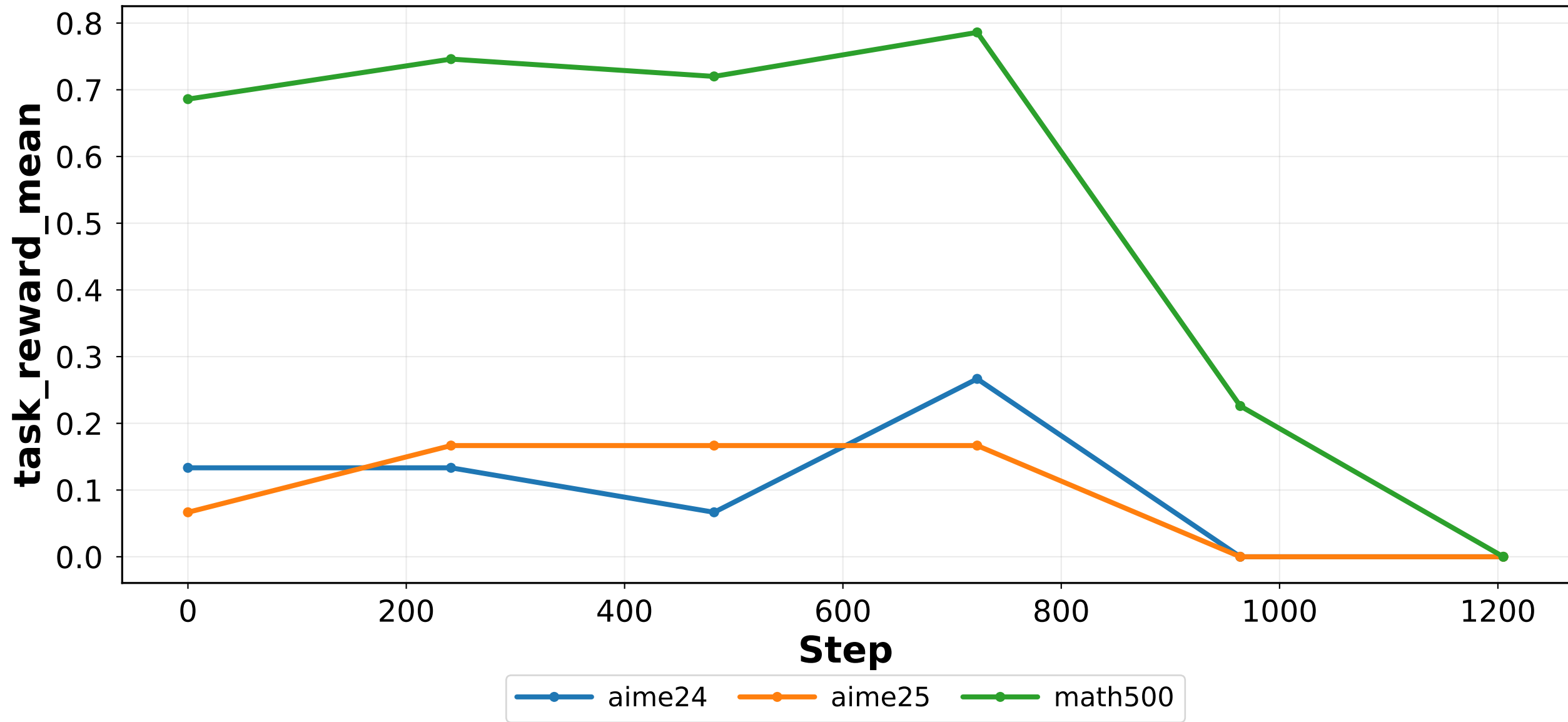
Evaluation Task Reward
